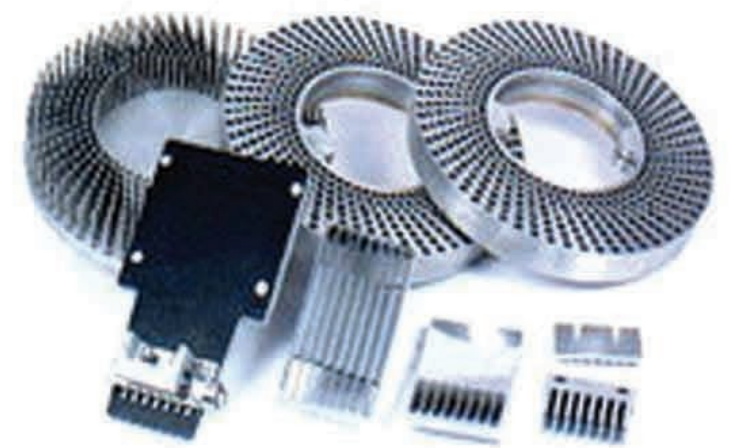
Capsule Filling Machine Change Pads
